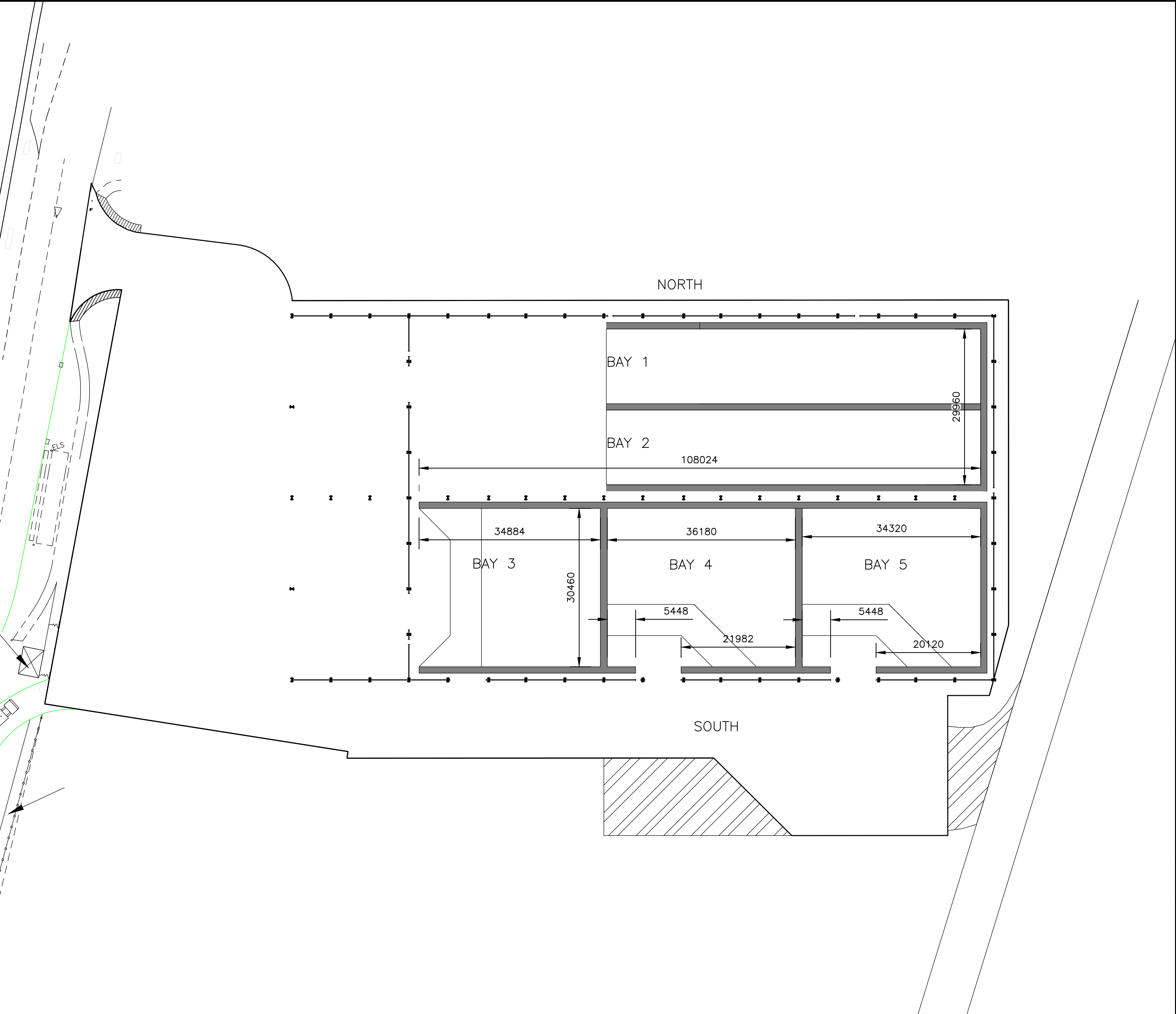
GENERAL ARRANGEMENT
